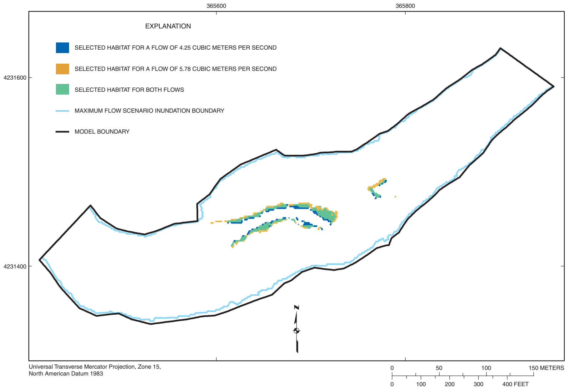
Figure 4-79. Selected habitat area distribution for habitat category 20 (flathead catfish) at flows of 4.25 and 5.78 cubic meters per second at Marais des Cygnes River site MDC2.
